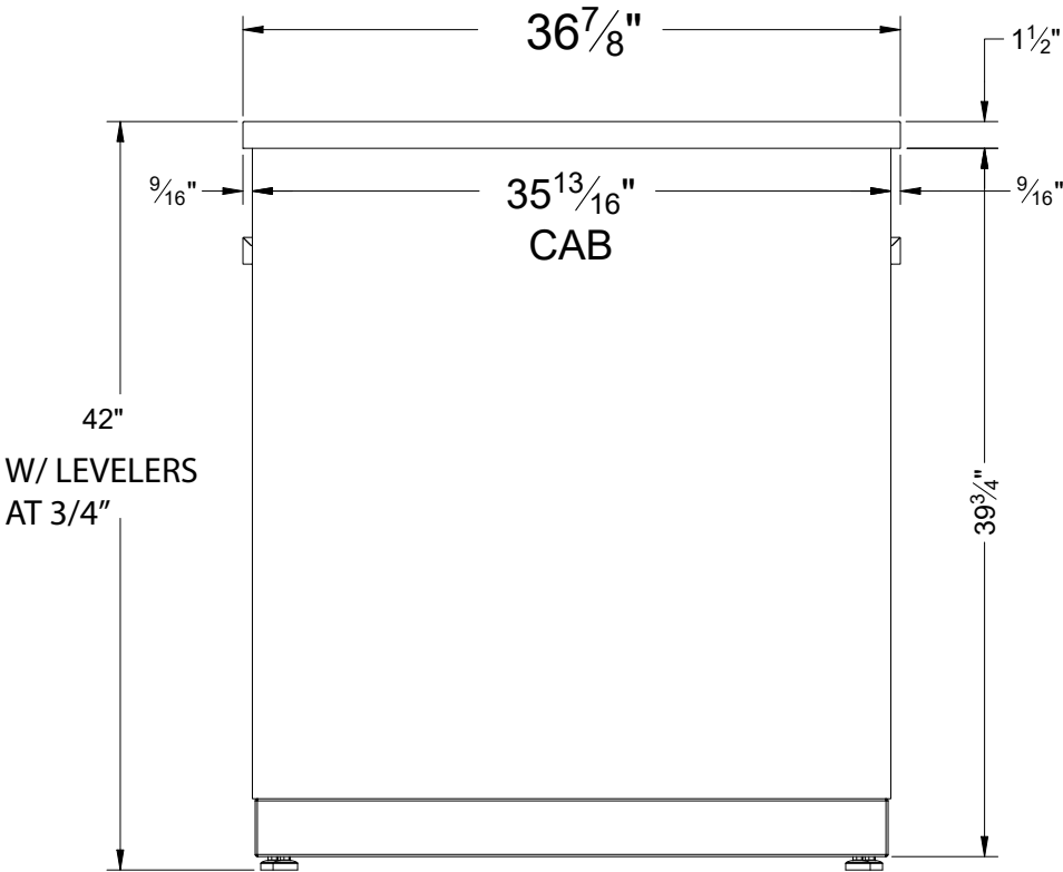
2 2 FRONT VIEW
