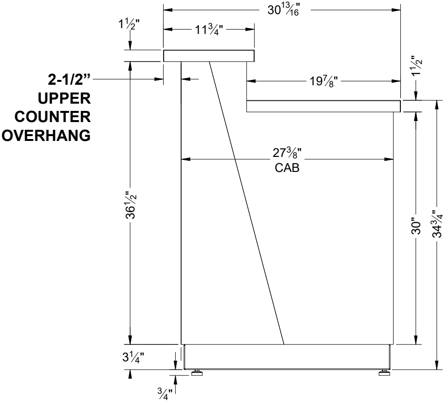
3 2 SIDE VIEW
